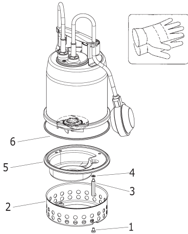
FIG. 8 • OPTIMA - BEST ONE - BEST ONE VOX
